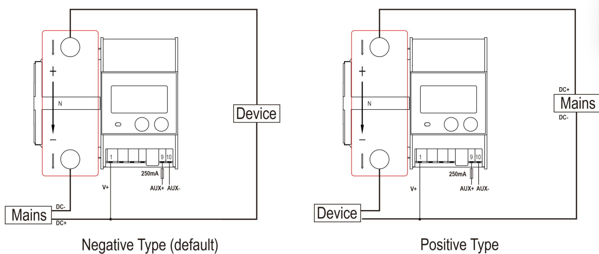
Wiring of the DCM6-650/-200 2-wire line loss mode (Figure6)
