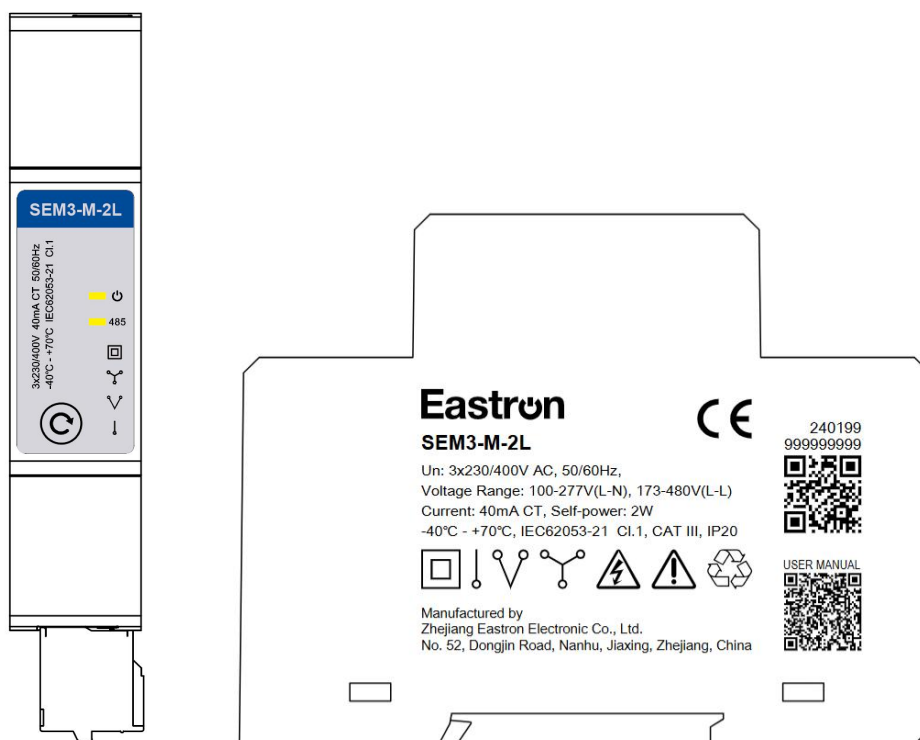
(SEM3-M-2L nameplate and laser printing)
