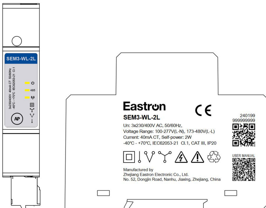
(SEM3-WL-2L nameplate and laser printing)
