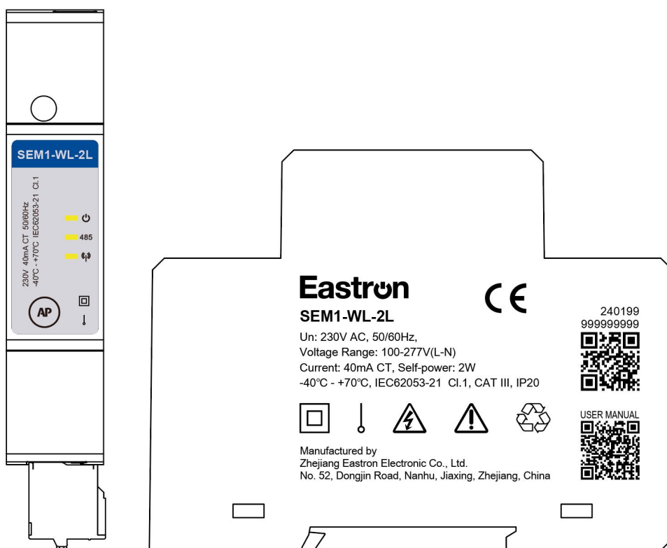
(SEM1-WL-2L nameplate and laser printing)
